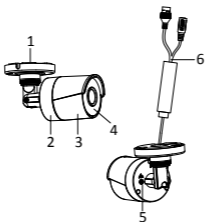
Figure 1-2 Type II Bullet Camera (PoE) Overview
